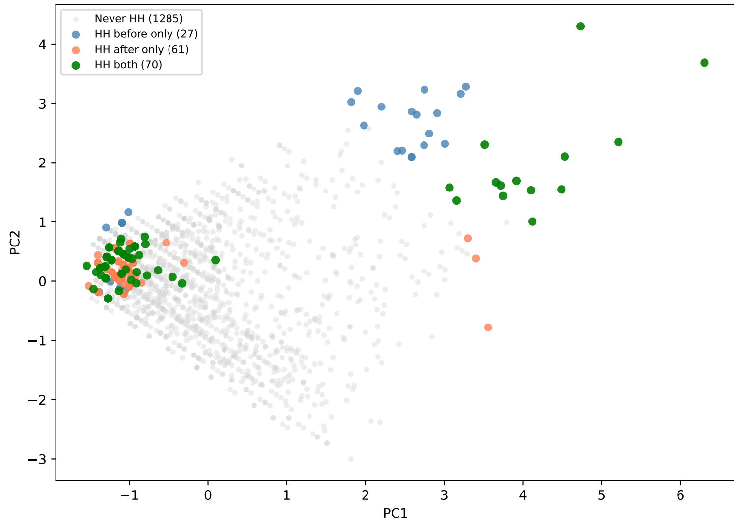
HH movement: before vs after platt calibration — compas (seed=6)
