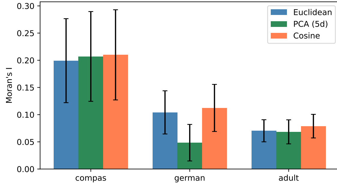
Moran's I
