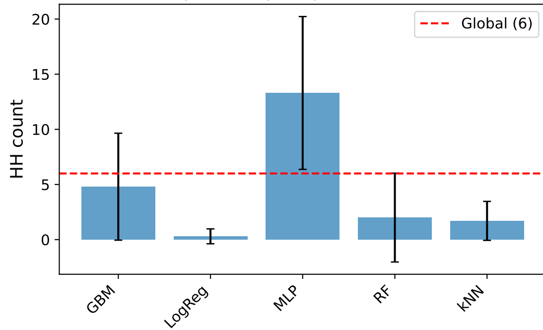
HH count: per-family vs global - German Credit
