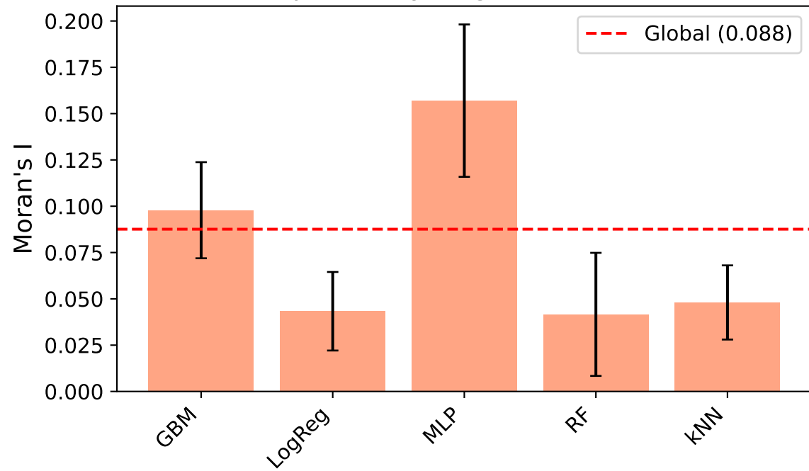
Moran's I: per-family vs global - German Credit
