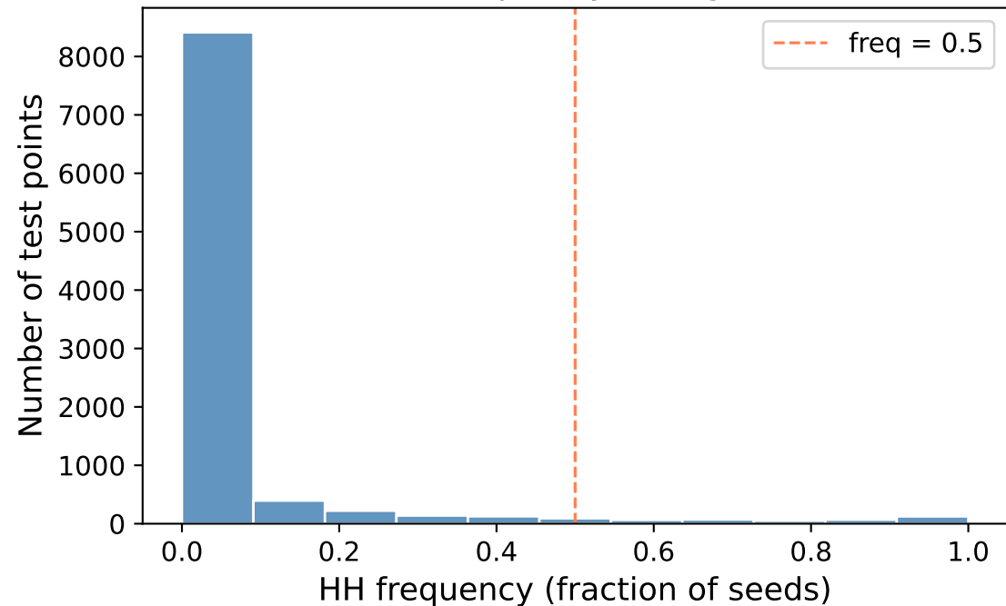
HH selection frequency histogram — Adult
