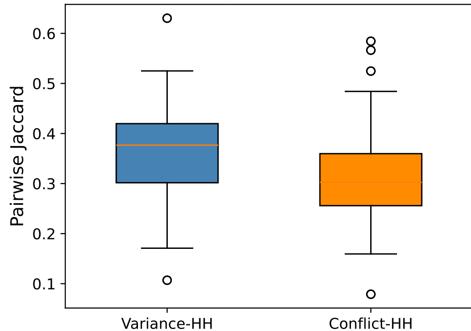
Pairwise HH Jaccard across seeds
