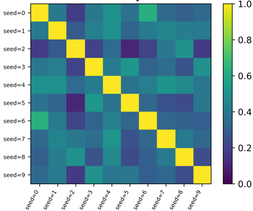
Variance-HH Jaccard
