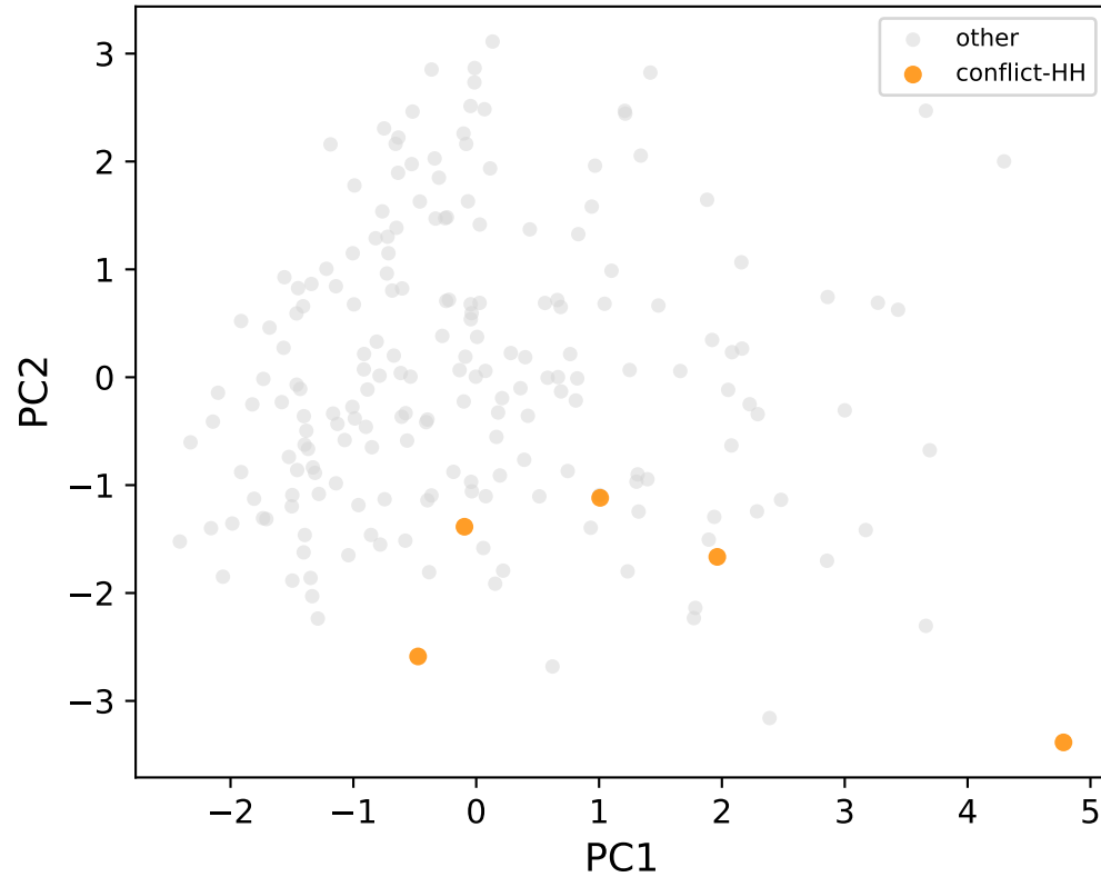
Conflict-HH — seed=3
