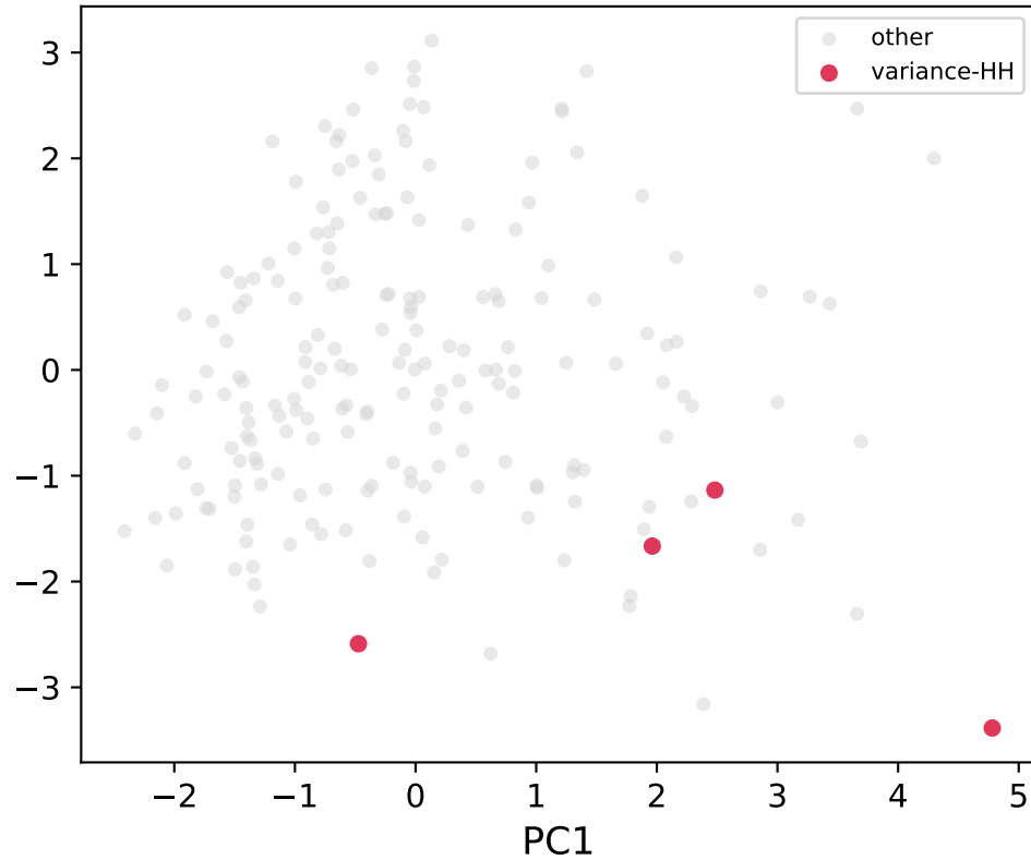
Variance-HH — seed=3
