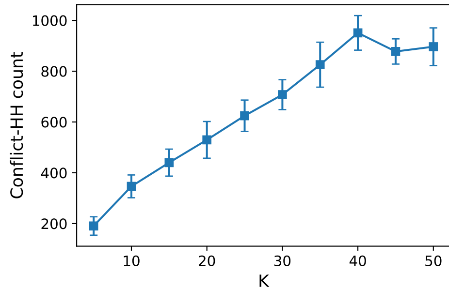
Conflict-HH count vs K
