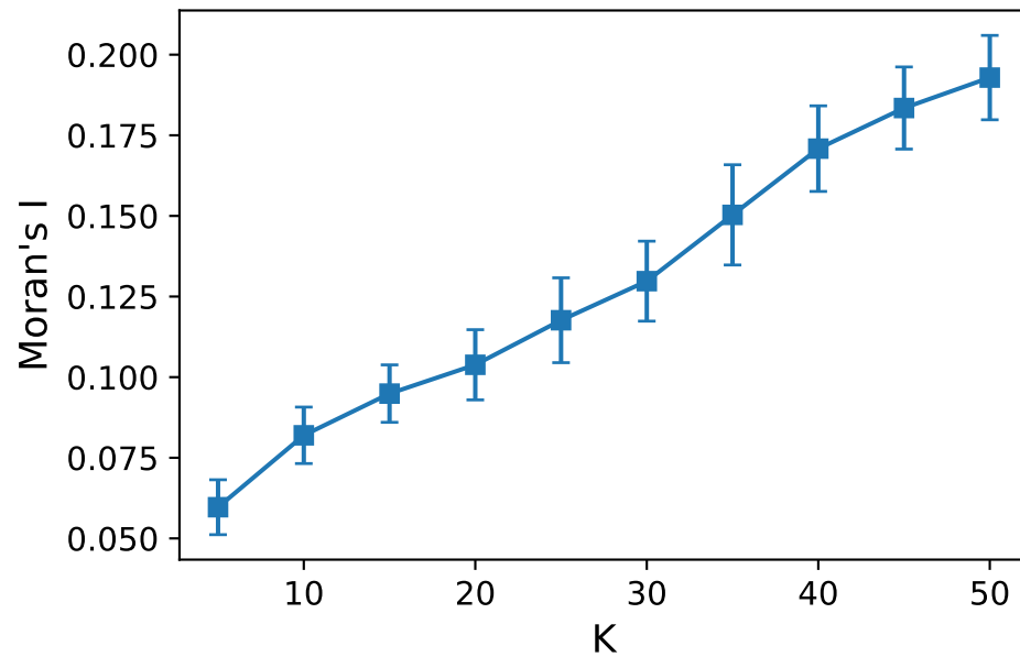
Conflict Moran's I vs K
