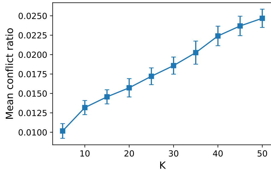
Mean conflict vs K
