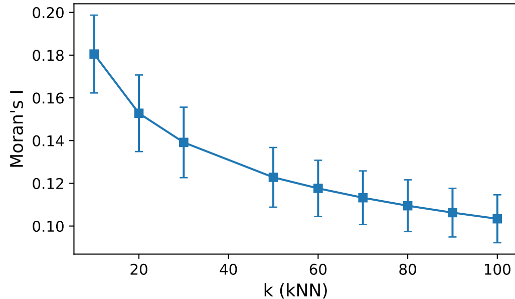
Conflict Moran's I vs k
