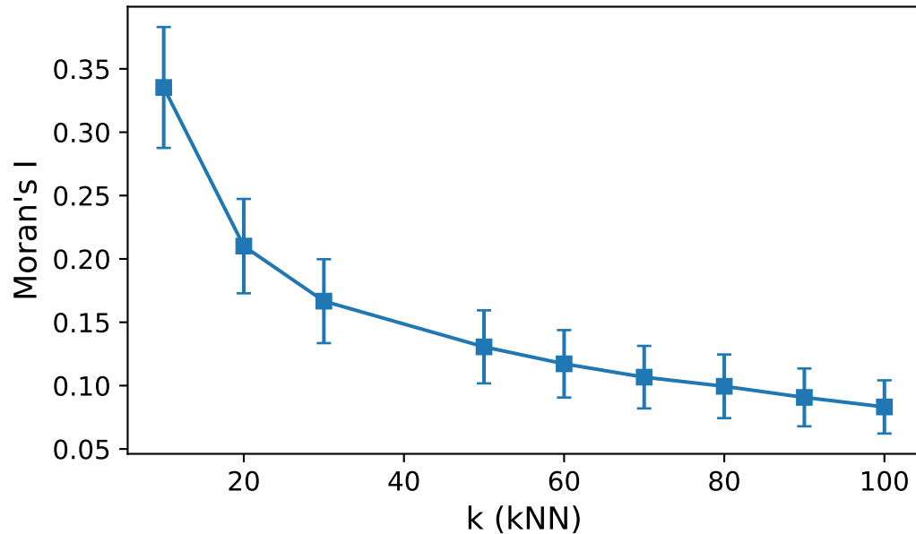
Conflict Moran's I vs k
