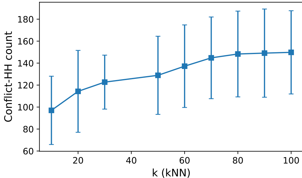
Conflict-HH count vs k
