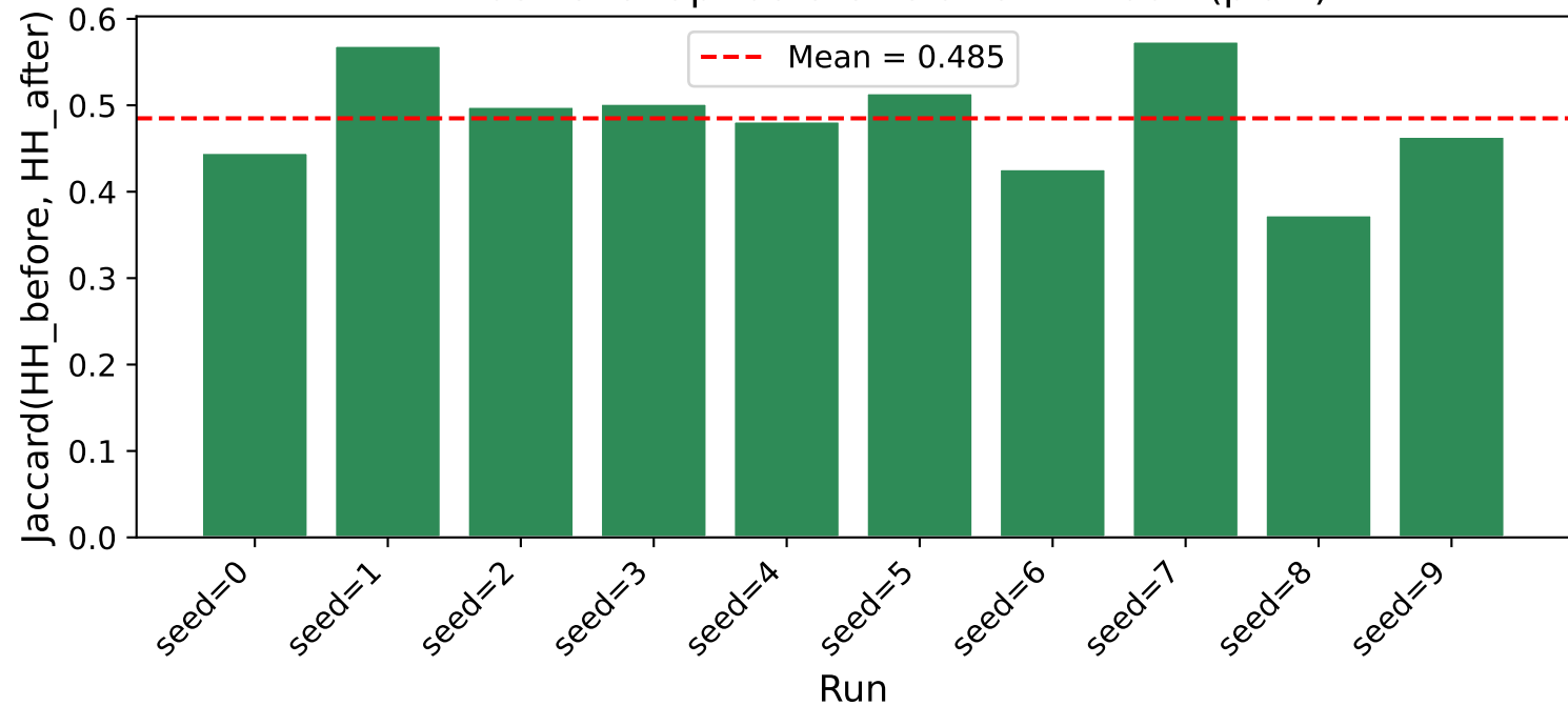
HH mask overlap: before vs after — Adult (platt)
