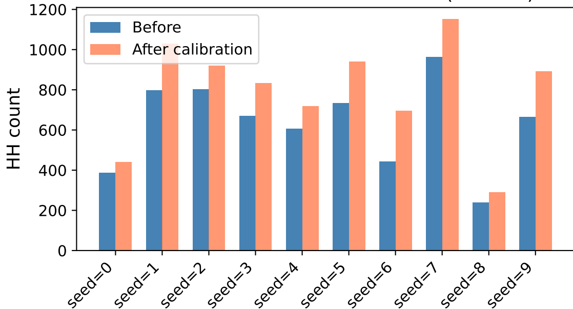
HH count: before vs after — Adult (isotonic)
