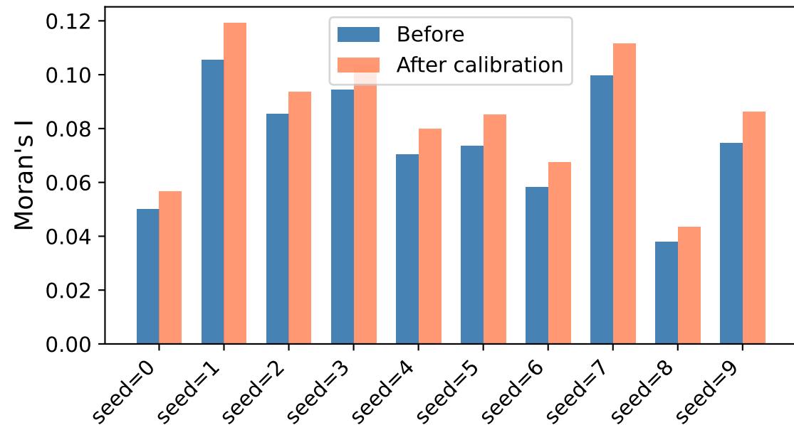
Moran's I: before vs after — Adult (isotonic)
