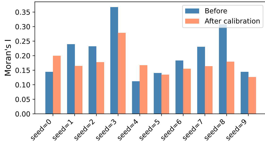
Moran's I: before vs after — COMPAS (isotonic)
