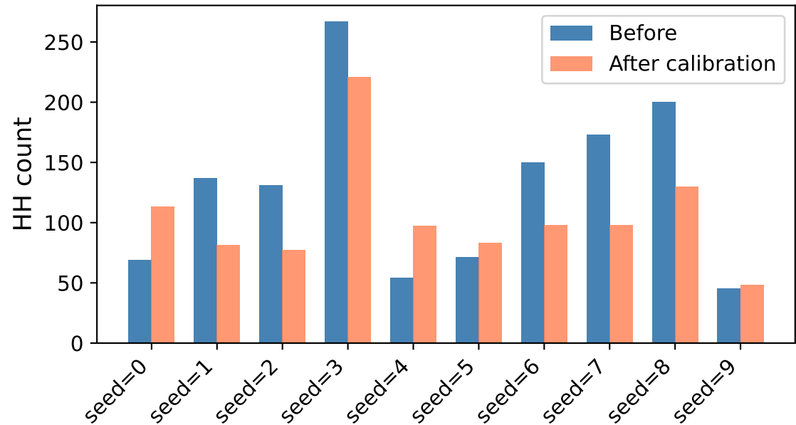
HH count: before vs after — COMPAS (isotonic)
