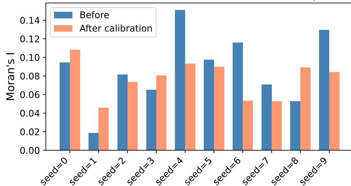
Moran's I: before vs after — German Credit (platt)
