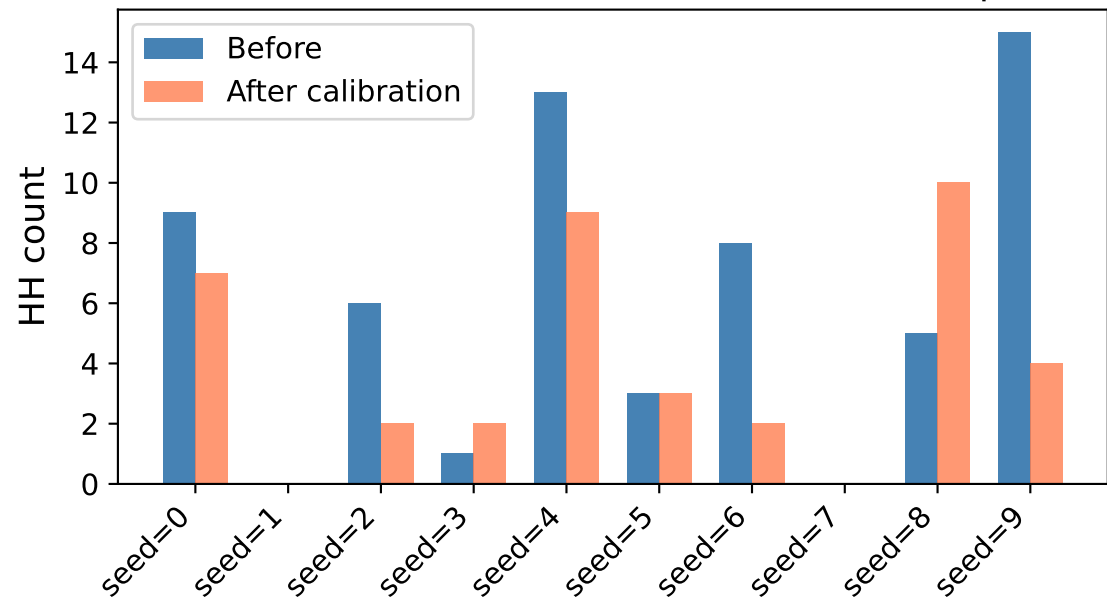
HH count: before vs after — German Credit (platt)
