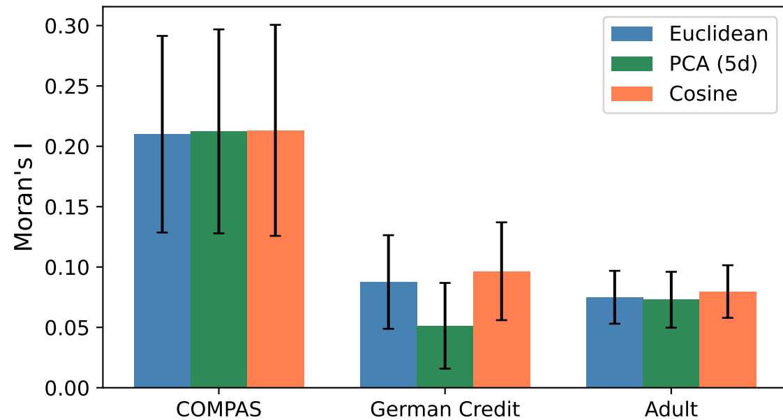
Moran's I
