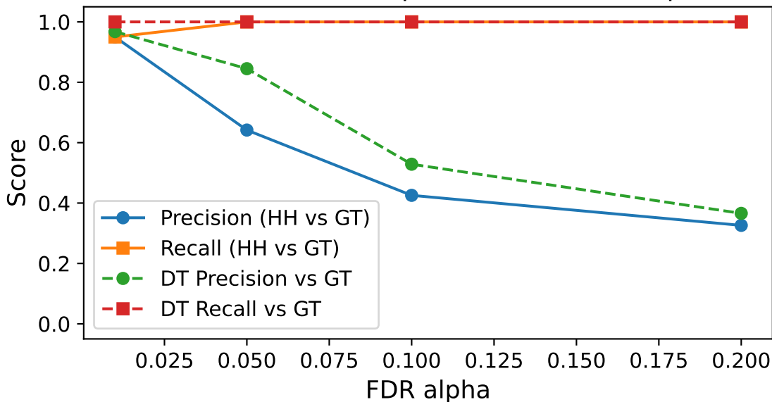
Precision & Recall vs alpha (structural exceptions)
