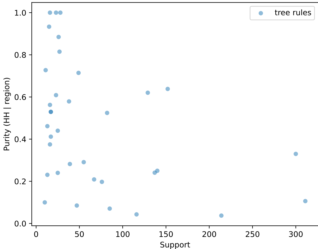
Tree rules: support vs purity (compas, all seeds)
