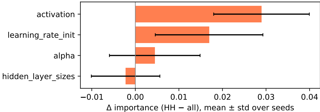
adult — MLP
