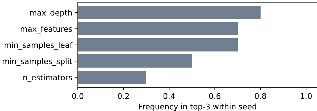
compas — RF: rank stability (subset=all)
