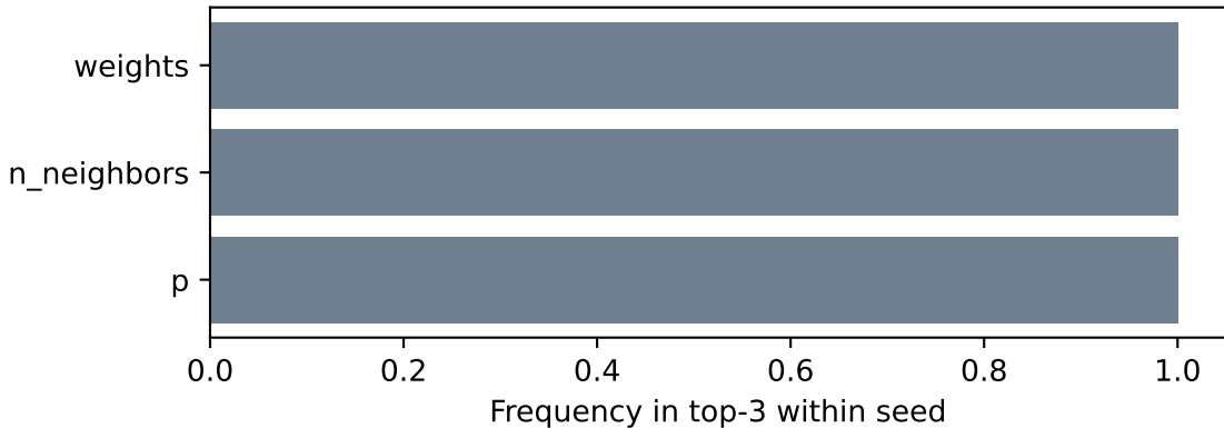
compas — kNN: rank stability (subset=all)
