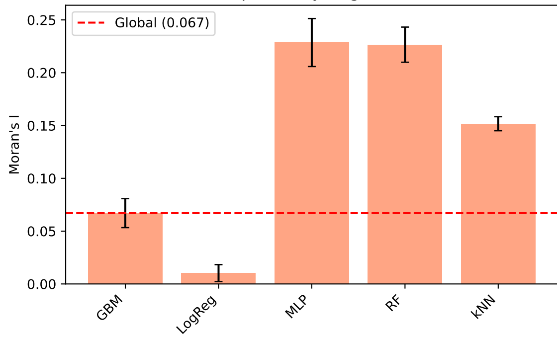
Moran's I: per-family vs global — adult
