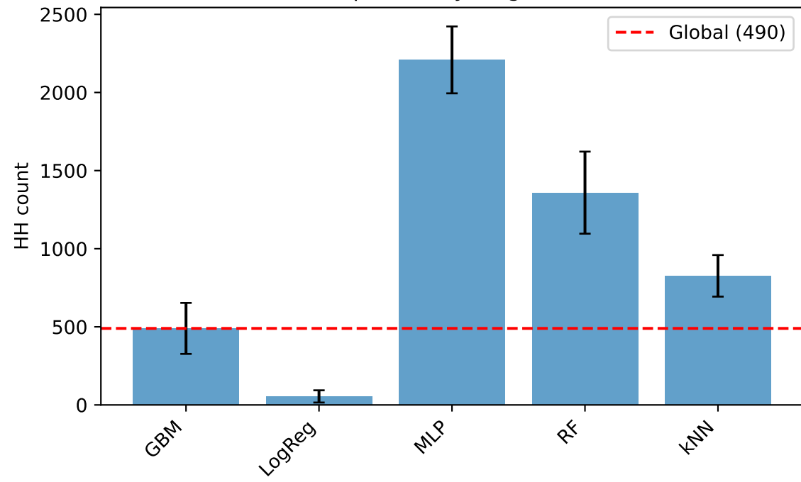
HH count: per-family vs global — adult
