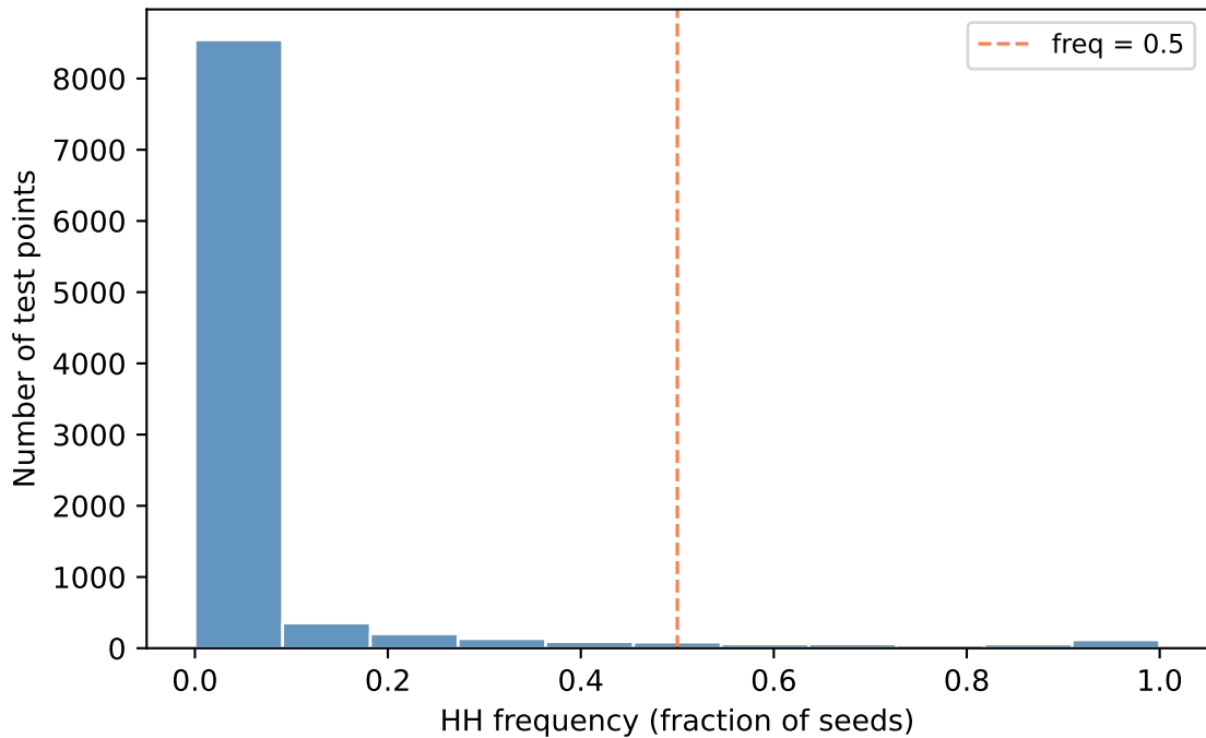
HH selection frequency histogram — adult
