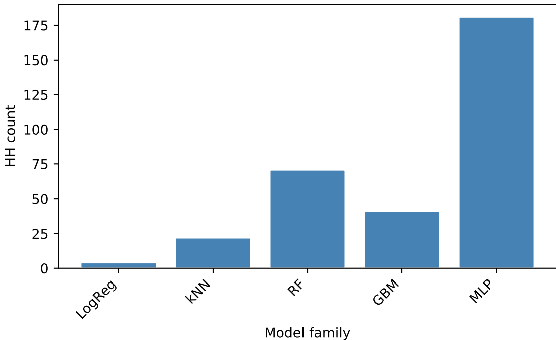
HH count by family (Compas, per-family top-25)
