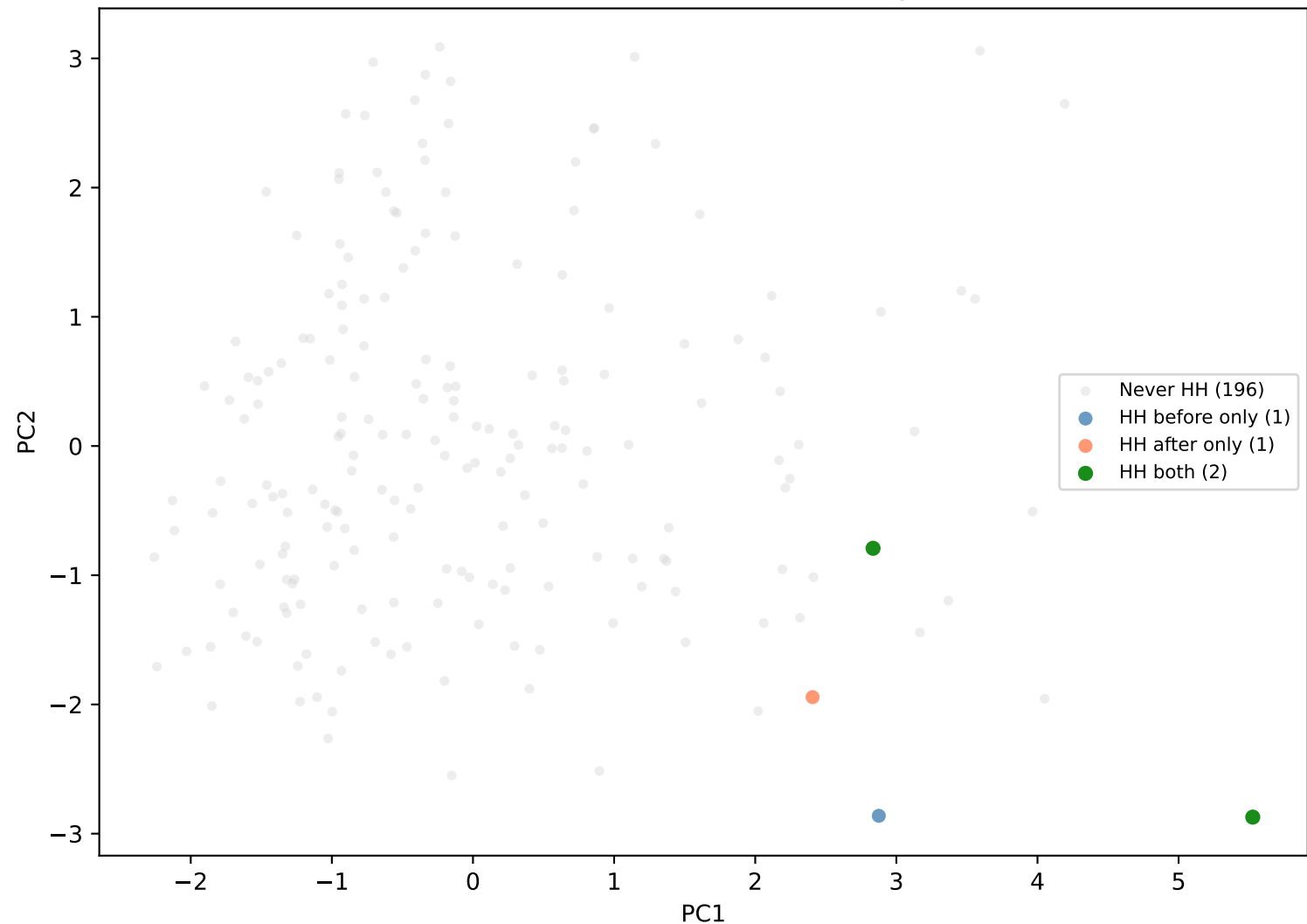
HH movement: before vs after calibration — german (seed=0)
