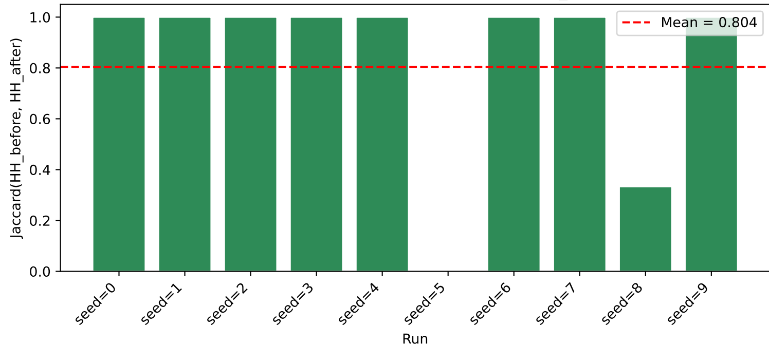
HH mask overlap: before vs after — breast_cancer
