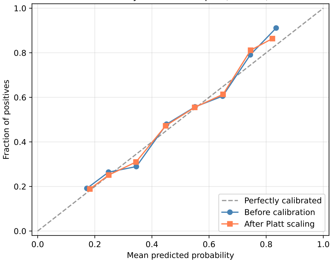
Reliability curve — compas (seed=6)
