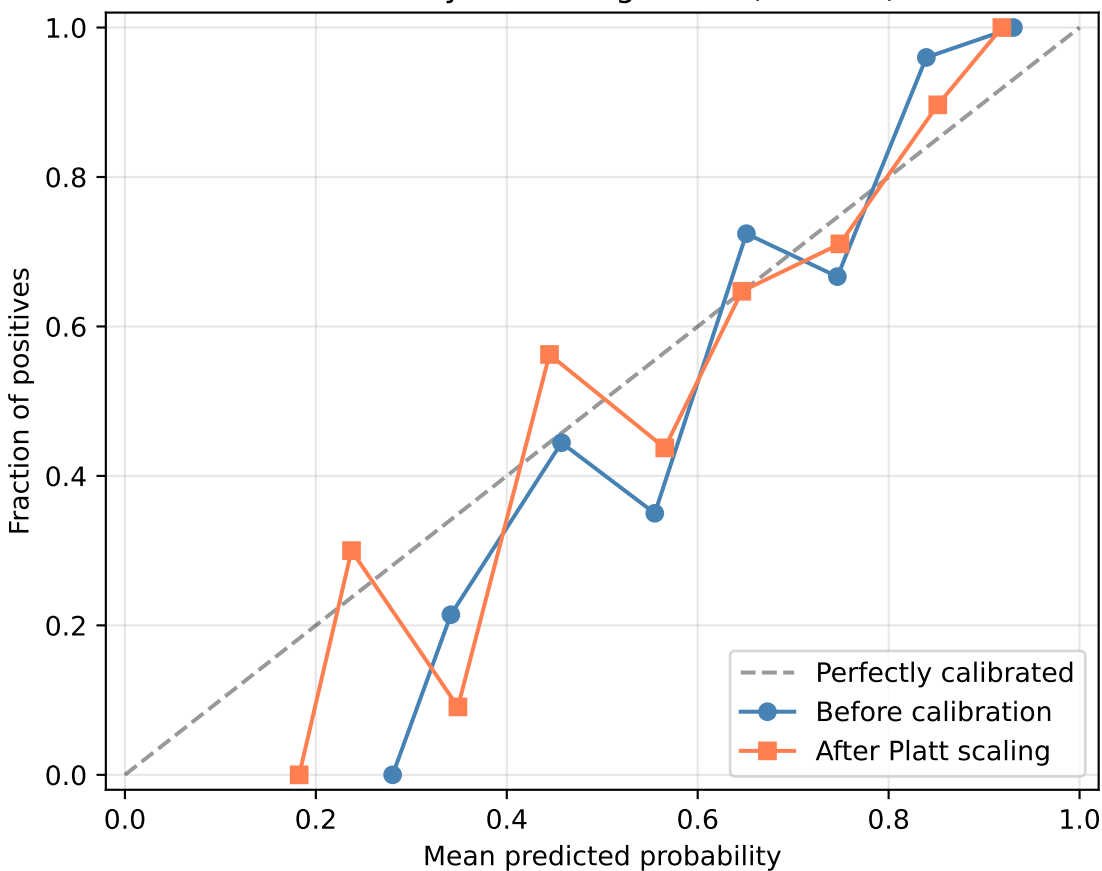
Reliability curve — german (seed=0)
