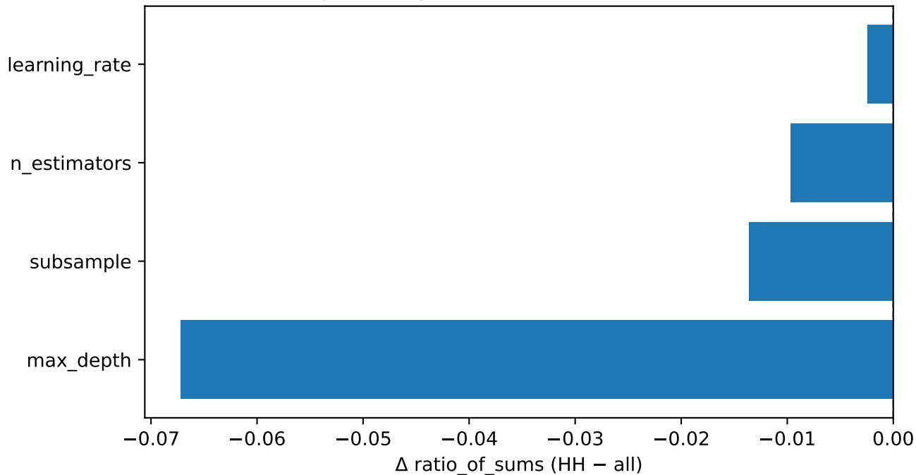
compas | seed 0 | GBM — HP importance shift in HH
