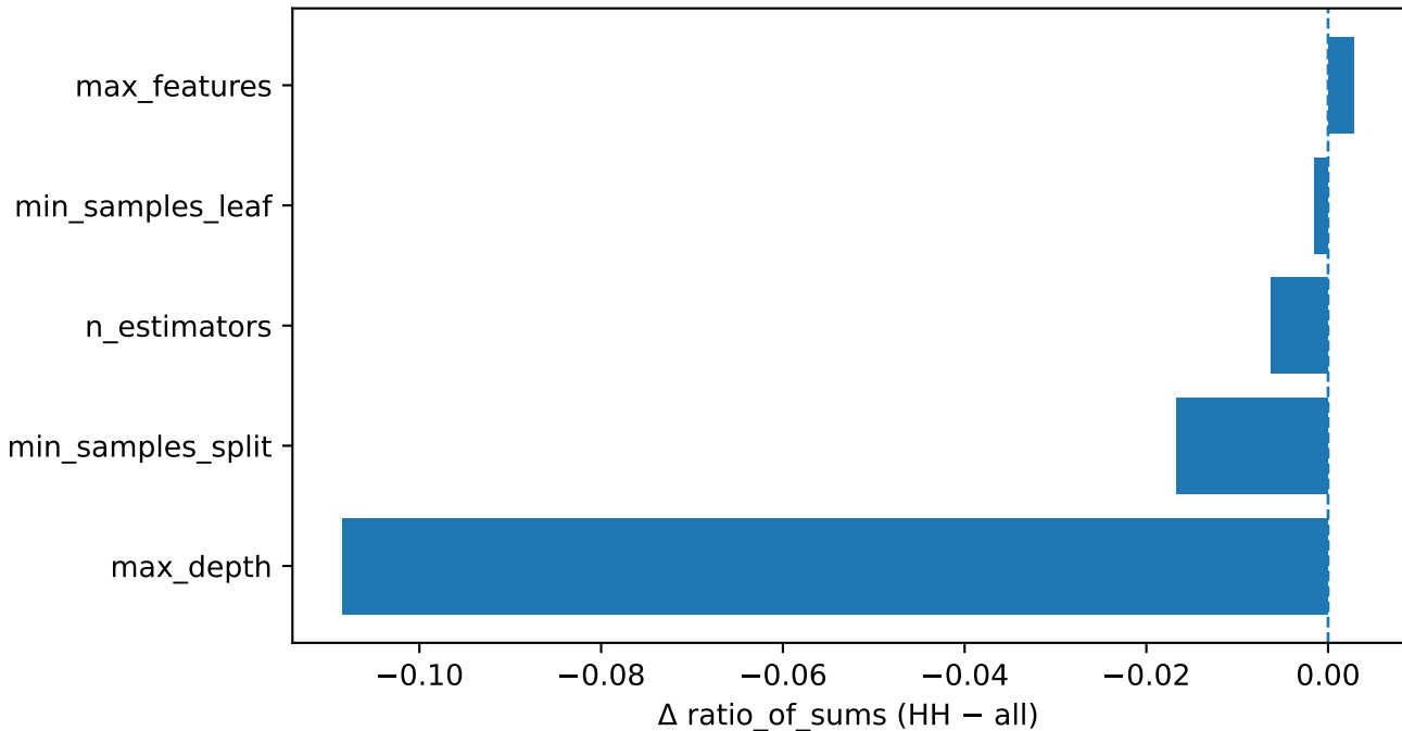
compas | seed 0 | RF — HP importance shift in HH
