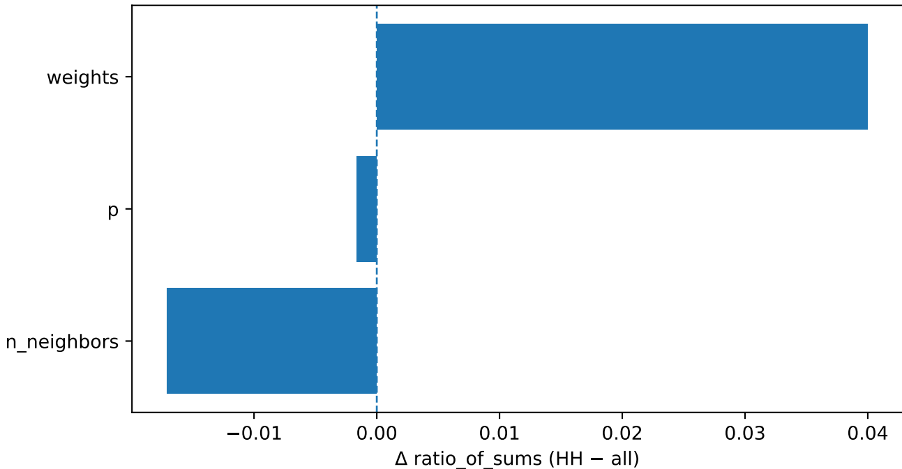
compas | seed 0 | kNN — HP importance shift in HH
