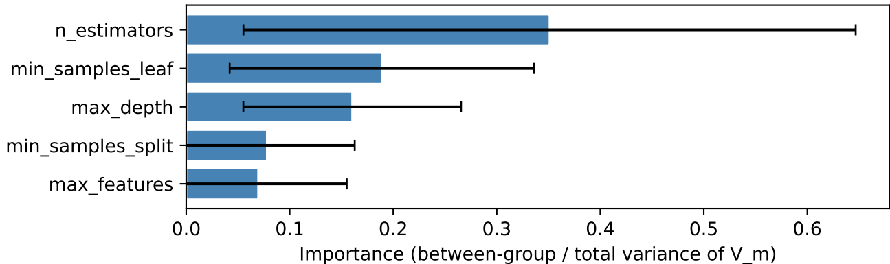
breast_cancer — RF: top HP importance (mean \pm std over seeds)
