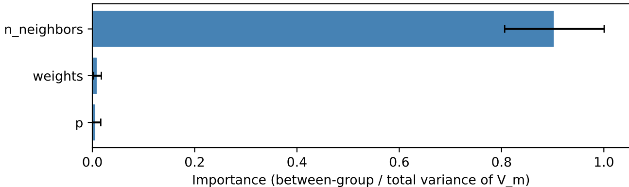
breast_cancer — kNN: top HP importance (mean \pm std over seeds)
