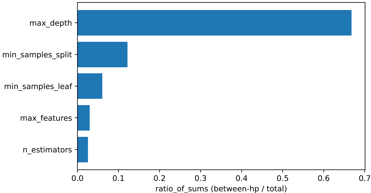
compas | seed 0 | RF — within-family HP importance
