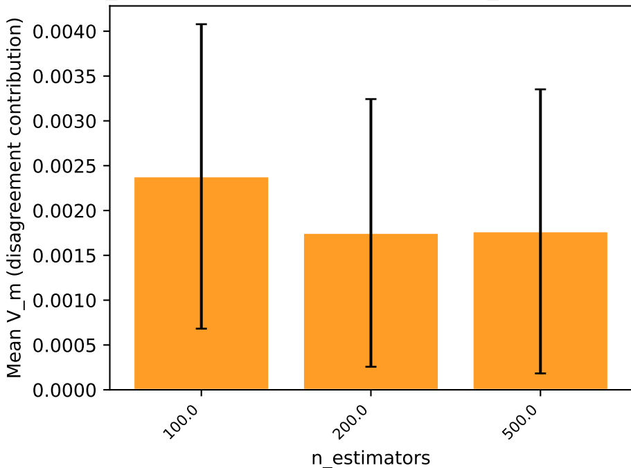
breast_cancer — RF: marginal effect of n_estimators on V_m
