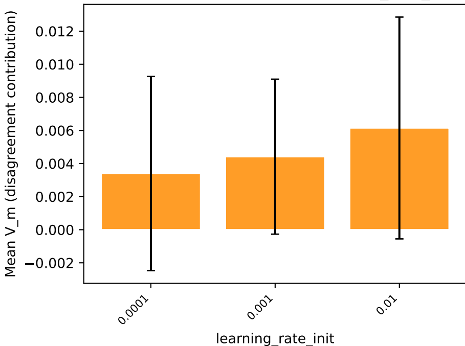
german — MLP: marginal effect of learning_rate_init on V_m
