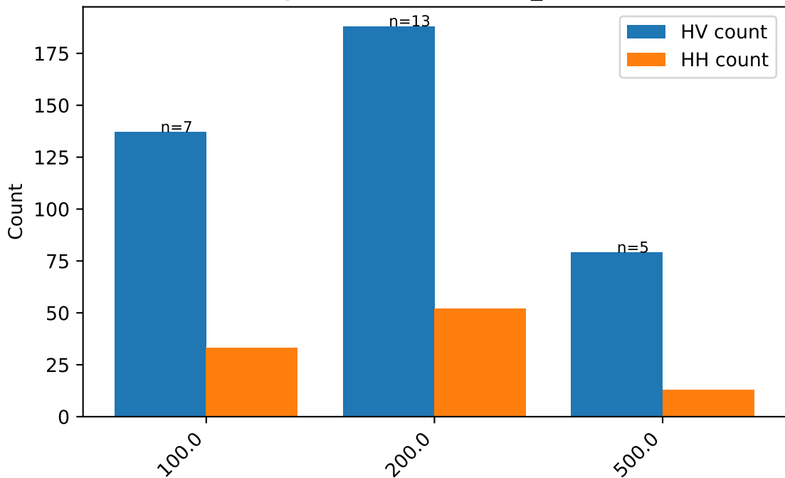
HP range effects: GBM \hat{\epsilon} n_estimators
