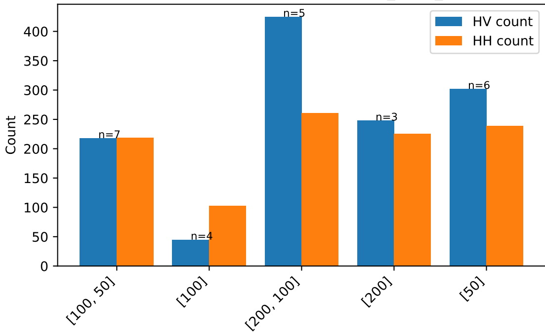
HP range effects: MLP " hidden_layer_sizes
