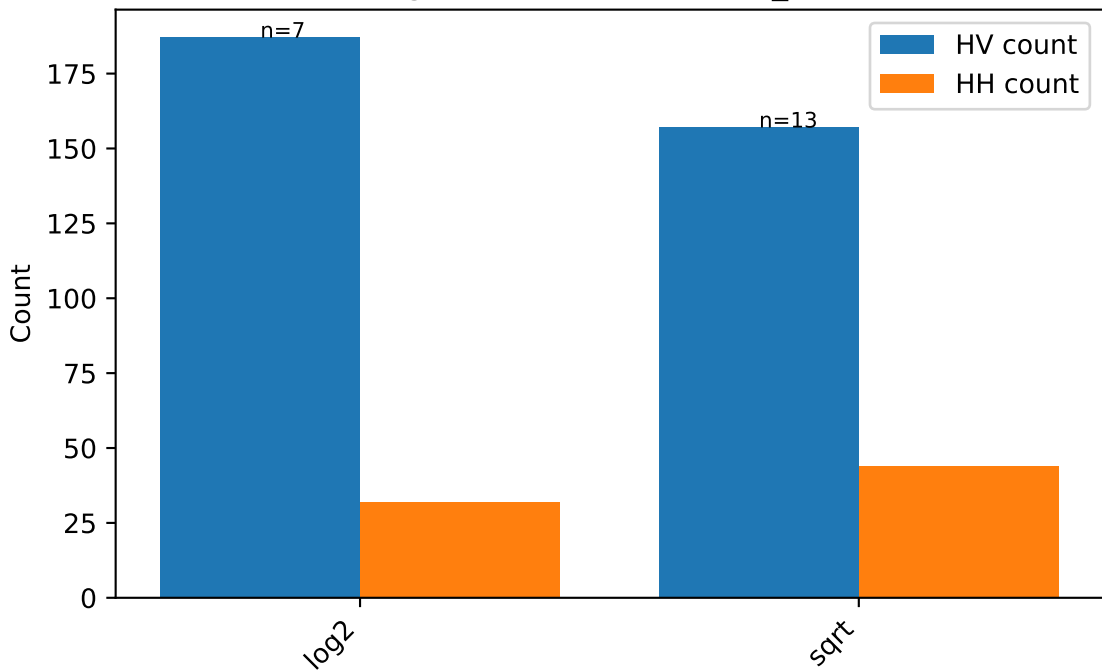
HP range effects: RF " max_features
