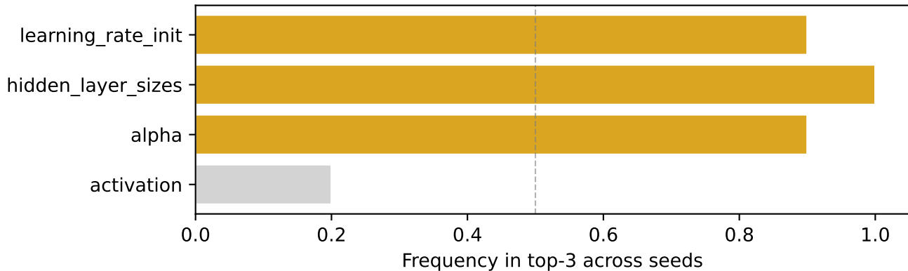
german — MLP: rank stability (top-3 frequency)
