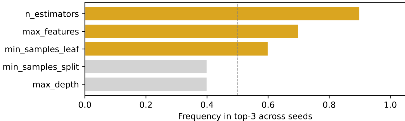
german — RF: rank stability (top-3 frequency)
