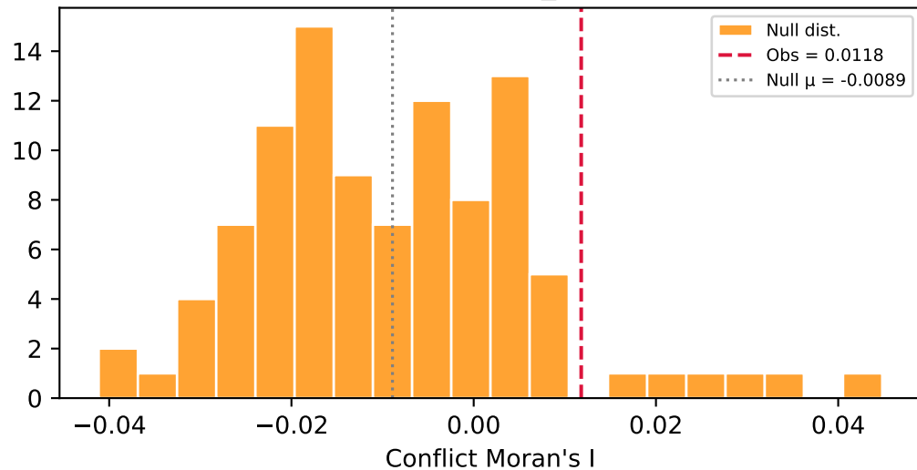
Conflict Moran's I (p_emp=0.069)
