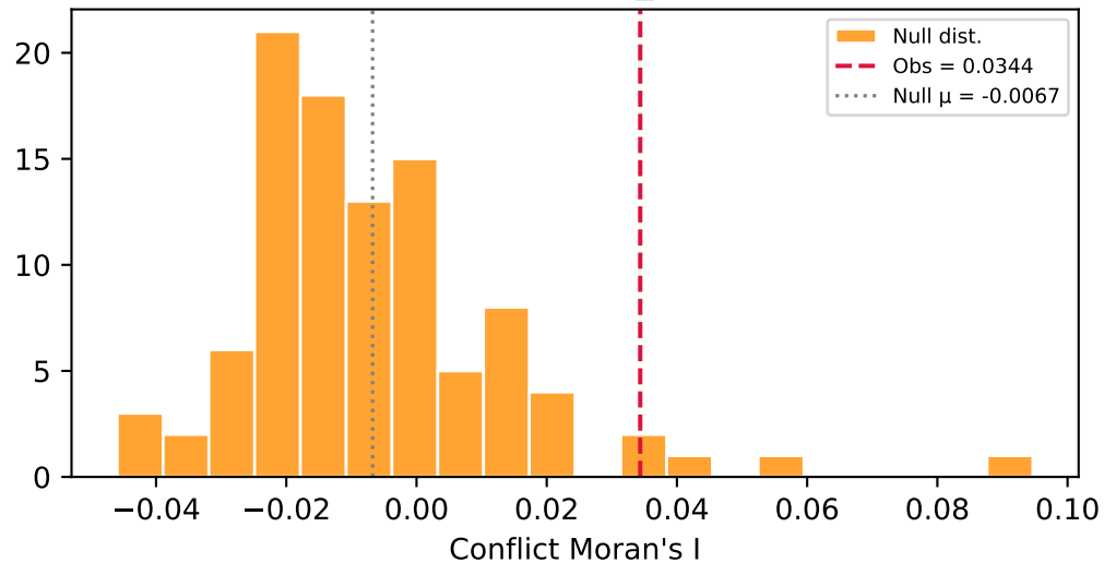
Conflict Moran's I ( p_{emp}=0.059 )
