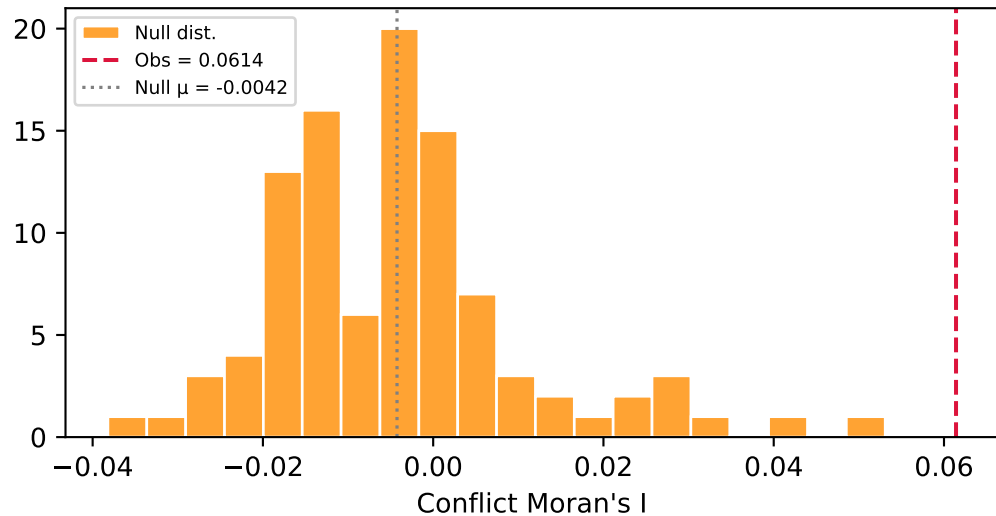
Conflict Moran's I (p_emp=0.010)
