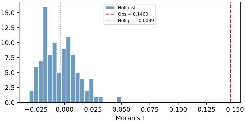
Moran's I (p_emp=0.010, p_pysal=0.001)
