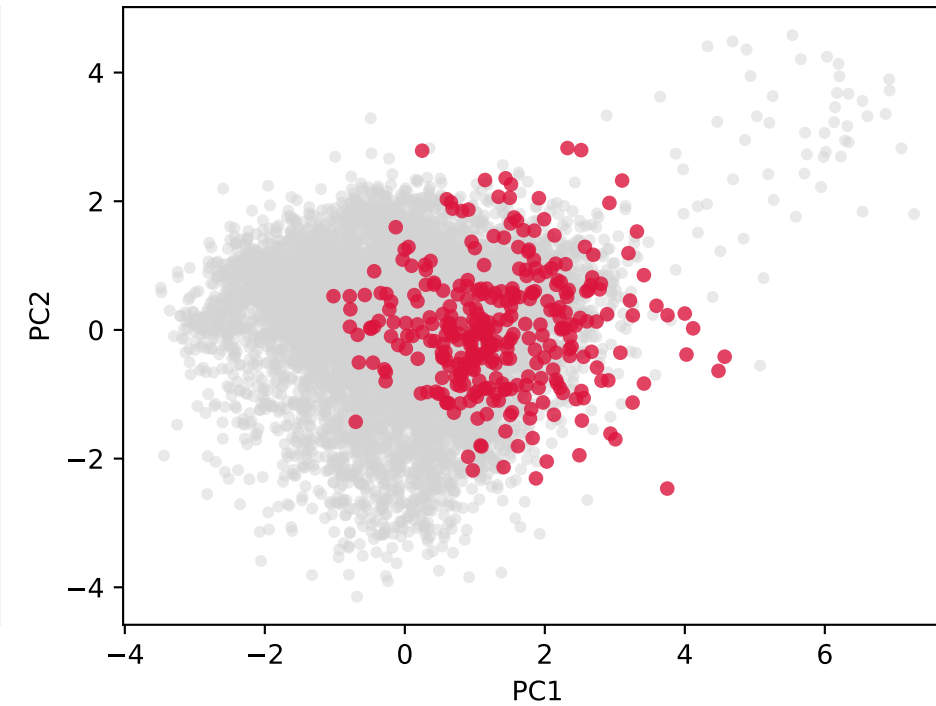
k=50, n_HH=326
