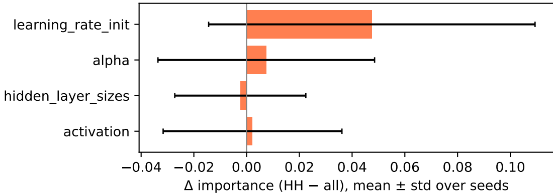
compas — MLP
