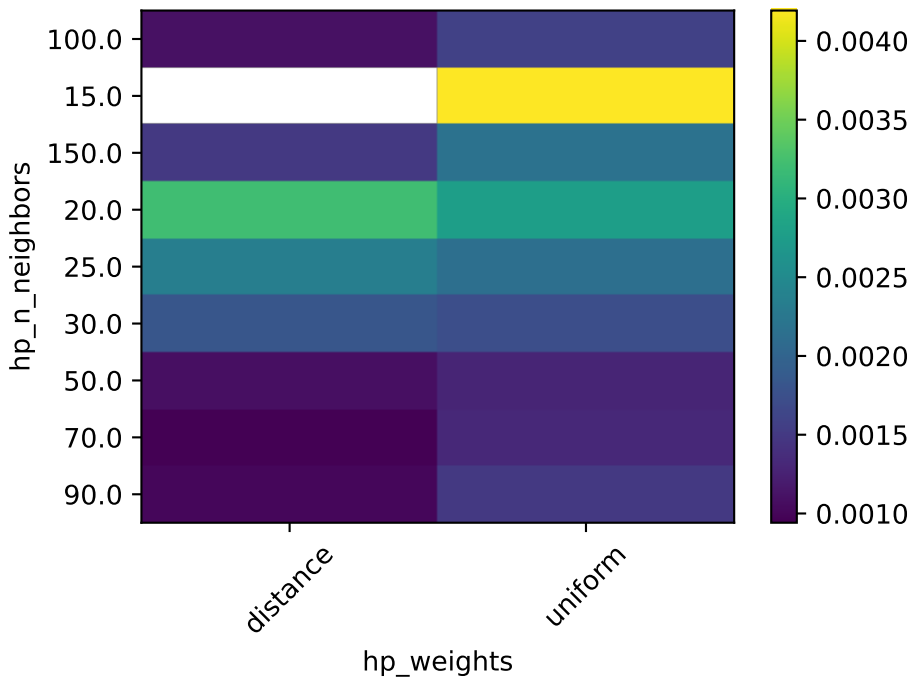
adult — kNN — Rashomon
