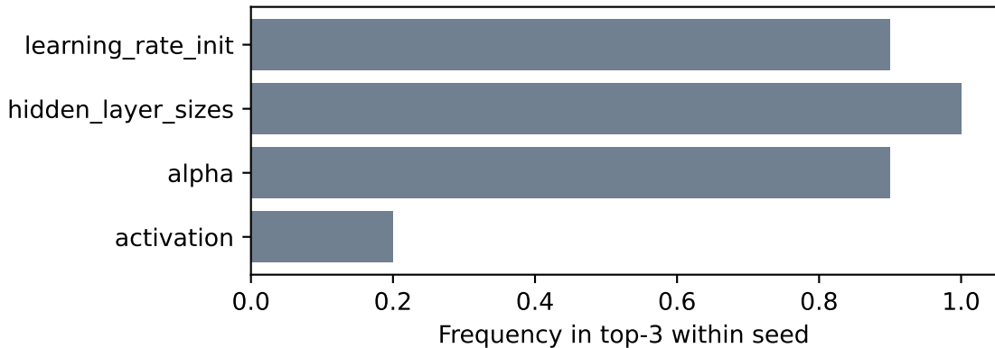
german — MLP: rank stability (subset=all)
