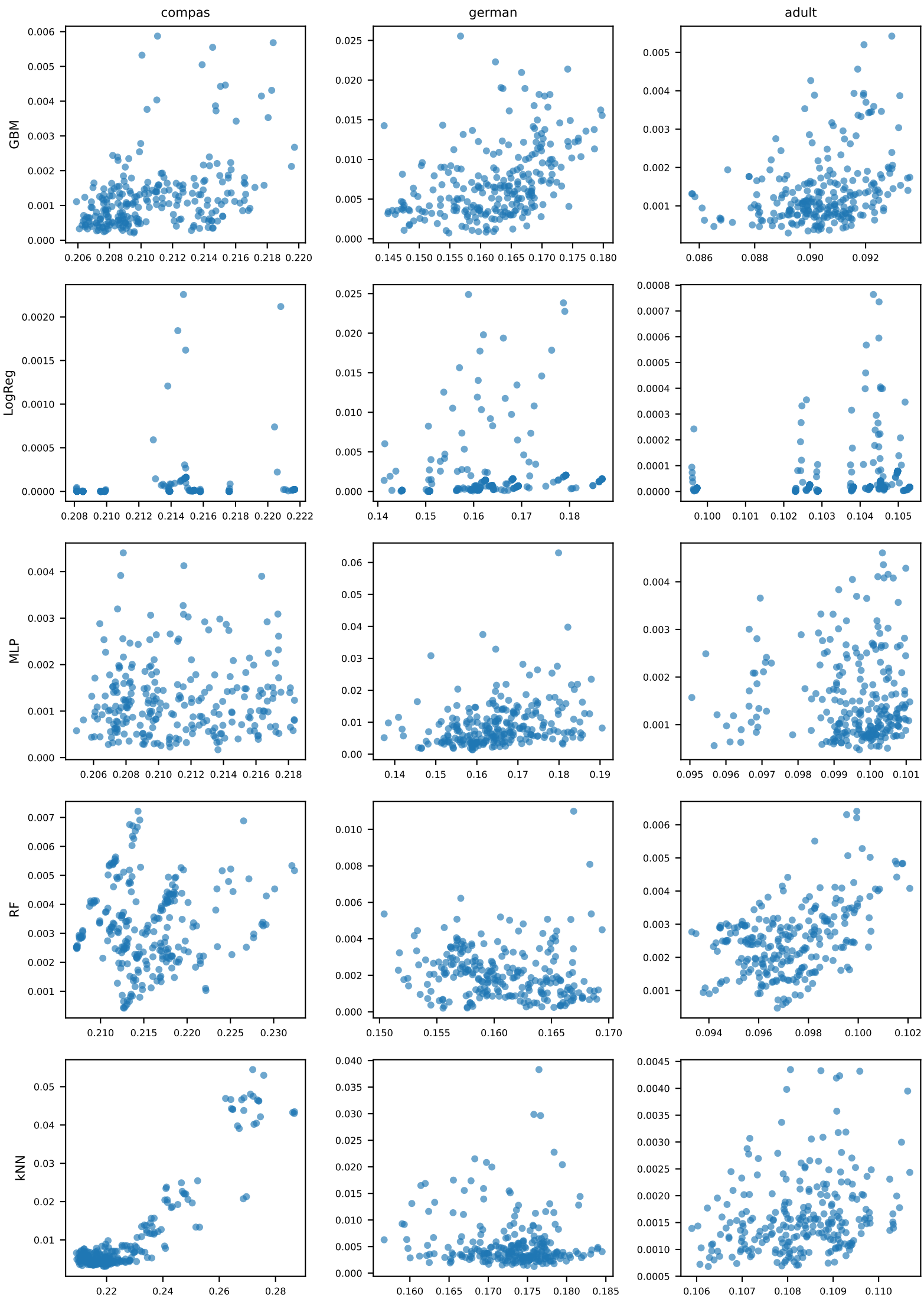
V_m vs validation Brier (Rashomon)
