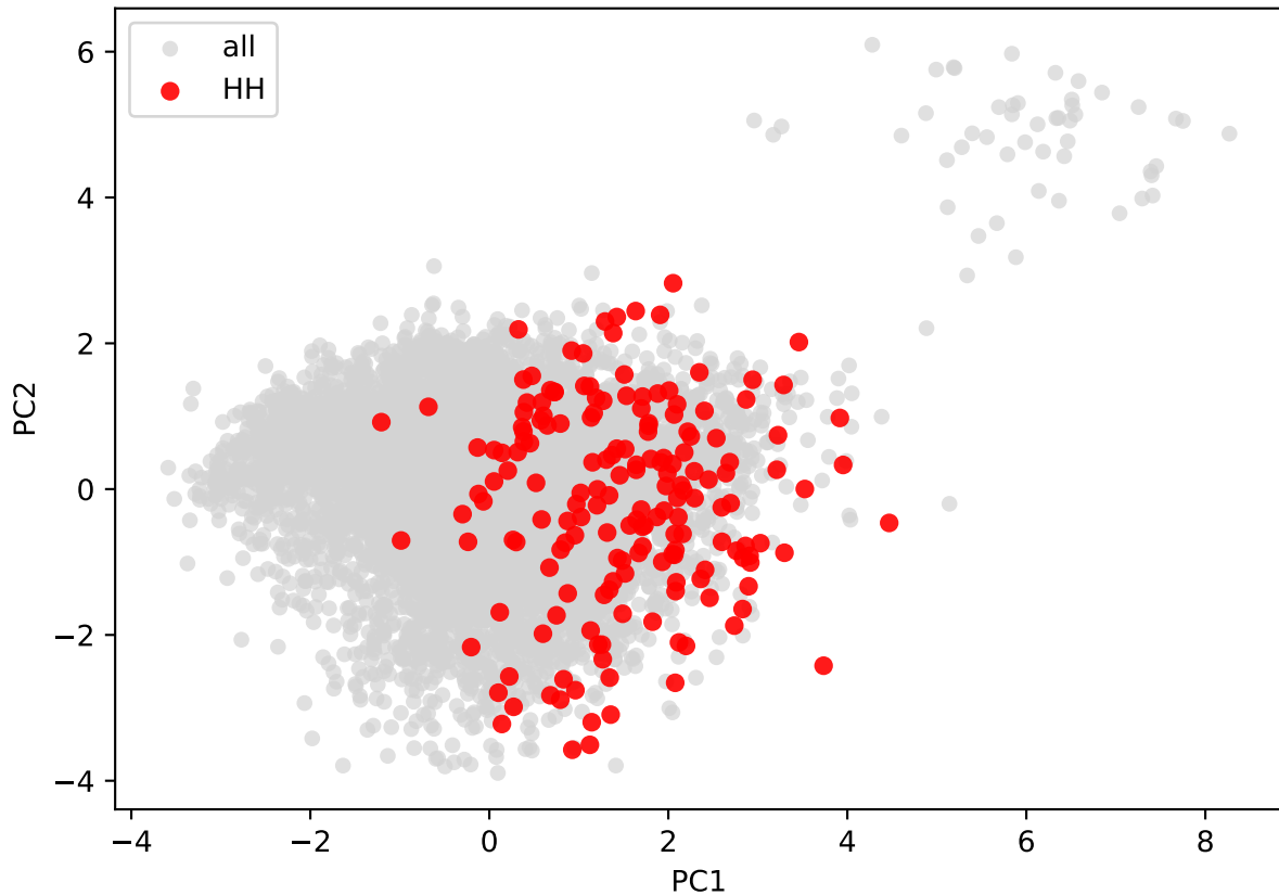
HH hotspots in feature space — seed=5
