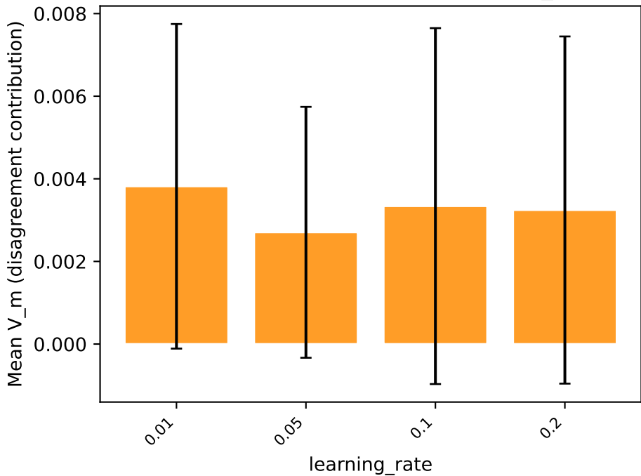
german — GBM: marginal effect of learning_rate on V_m
